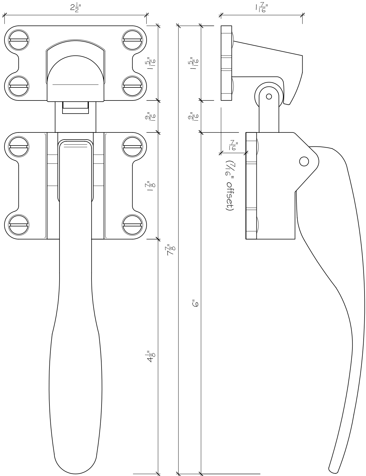
TRADITIONAL ICE BOX LATCH
